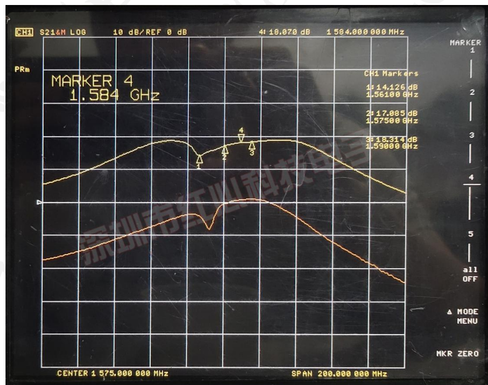
(Gain)增益图
