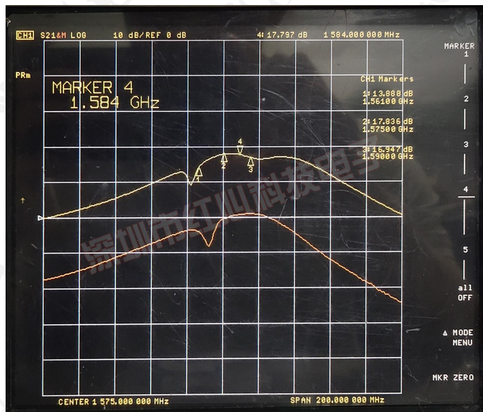
(Gain)增益图
