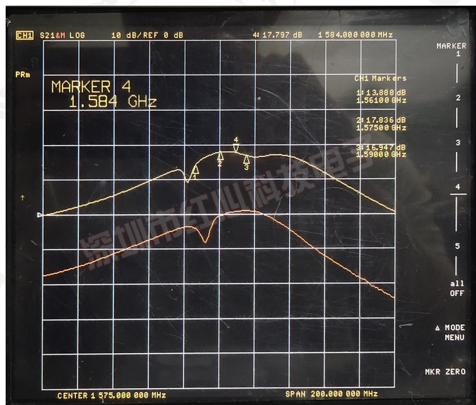
(Gain)增益图
